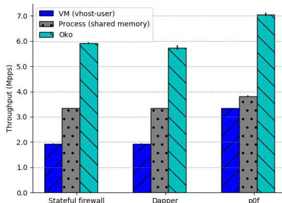
Figure 8: Comparison of performance for the three use cases, with Oko, a vhost-user KVM virtual machine, and a DPDK Ring Port process. The standard deviation is below 0.10 for all measurements.
