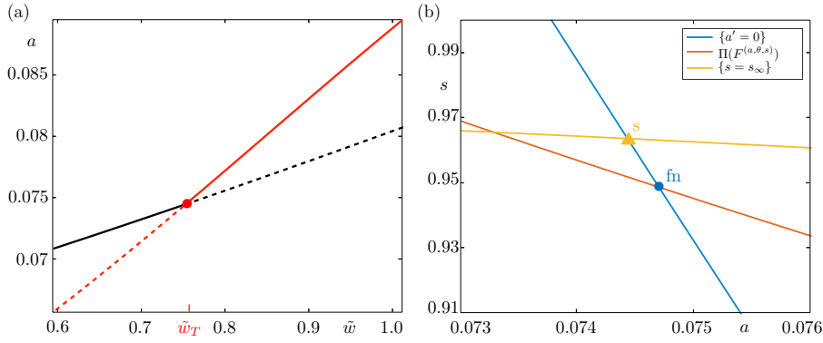
Fig. 8 (a) Bifurcation diagram of (12) with respect to \tilde{w} . Solid (resp. dashed) lines correspond to stable (resp. unstable) equilibria, and both branches cross at \tilde{w}_T = 0.754645 , where they exchange stability via a transcritical bifurcation (marked by a red dot); note that the branch plotted in red corresponds to the projection of the fold curve onto the (a, s) -plane. (b) Phase portrait of (12) for \tilde{w} = 0.7625 . The node equilibrium corresponds to a folded node fn for the reduced system, with coordinates (a_{fn}, s_{fn}) \approx (0.074696, 0.94875) ; it lies at the intersection between the a -nullcline (blue) and the projection \Pi(F^{(a,\theta,s)}) of the fold curve onto the (a, s) -plane (red). The saddle equilibrium s , with coordinates (a_s, s_s) \approx (0.074426, 0.96368) , lies at the intersection between the a -nullcline (blue) and the \{s = s_\infty\} -component of the s -nullcline (yellow).
