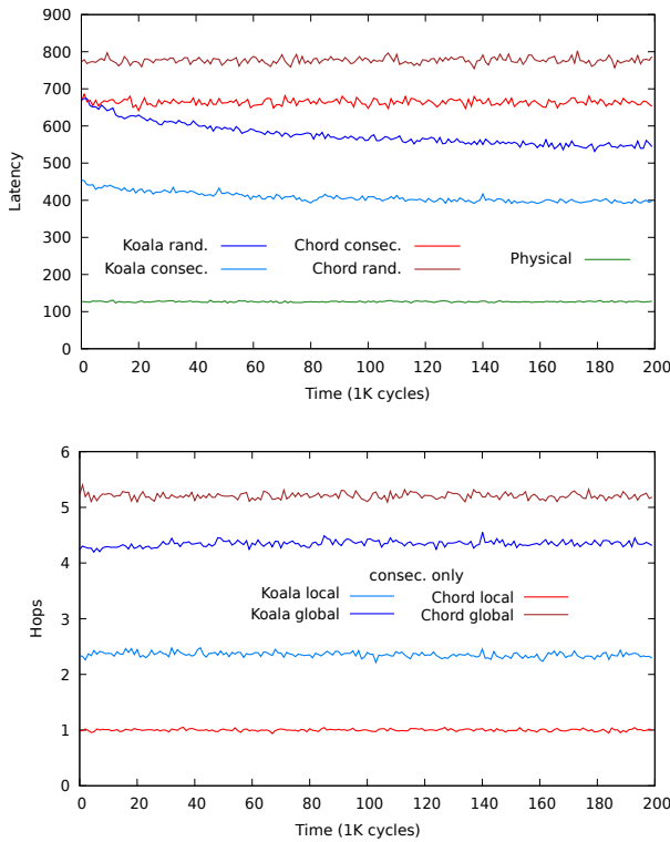
Fig. 8: Impact of cloud topology on Koala and Chord.
