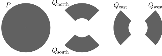
Fig. 1. Pupil geometries used to compute sound-speed or source kernels ( P ) and flow kernels ( Q ), also see Table 2.
