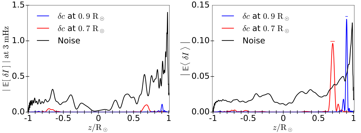
Fig. 4. Left panel: Hologram intensity |\mathbb{E}[\delta I_{\alpha\beta}(x)]| at a single frequency of 3 mHz, displayed along the z -axis (at x = z\hat{\mathbf{z}} ). The sound-speed perturbation (see Eq. 54) is placed at two different positions along the z -axis, z_s = 0.7 R_\odot (red) and 0.9 R_\odot (blue). The standard deviation of the noise \sqrt{\text{Var}\langle I_{\alpha\beta,0}(x) \rangle} is given by the black curve. Note that the jagged aspect of the curves is not due to numerical inaccuracies. Right panel: hologram intensity and noise level after averaging over 101 frequencies uniformly distributed in the interval from 2.75 to 3.25 mHz. The frequency resolution is 5 \mu\text{Hz} , implying an observation duration of T = 55.5 h. A horizontal line segment is plotted at each depth to mark half of the local wavelength.
