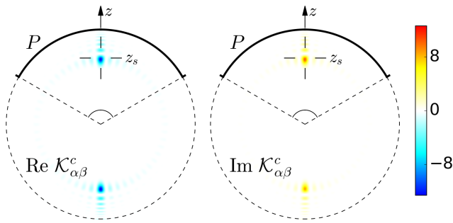
Fig. 9. Meridional slice of the sound-speed kernel \mathcal{K}_{\alpha\beta}^c with z_s = 0.7 R_\odot computed at the low frequency of 2.4000 mHz, which corresponds to the spike with a red dot in Fig. 7. This kernel displays oscillations and is not peaked as much as the 3-mHz kernel from Fig. 2.
