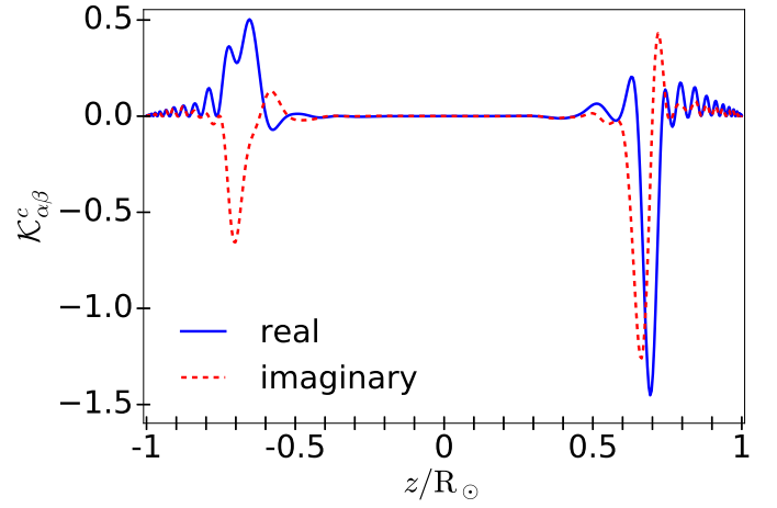
Fig. 3. Cut along the z axis through the sound-speed kernel from Fig. 2. The scatterer is at z_s = 0.7 R_\odot .
