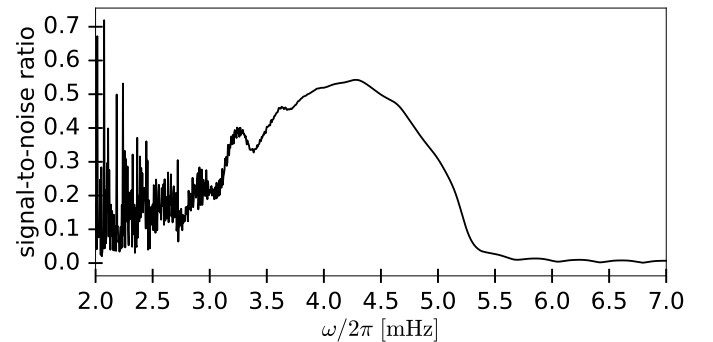
Fig. 8. Signal-to-noise ratio as in Fig. 7, but for a sound-speed scatterer located closer to the surface at z_s = 0.9 R_\odot .
