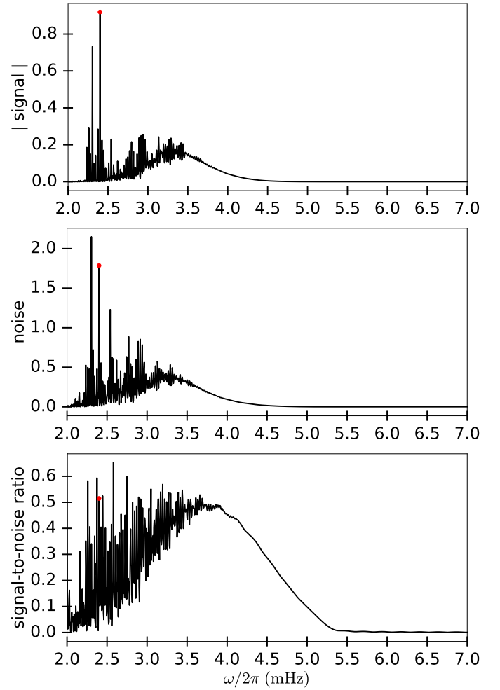
Fig. 7. Signal, noise, and signal-to-noise ratio as function of frequency for a sound-speed scatterer located at z_s = 0.7 R_\odot . Here we show the result for a frequency range of 2 to 7 mHz. The rapid changes are not due to numerical inaccuracies. The red dots mark the spikes in the signal and the noise at 2.4000 mHz.
