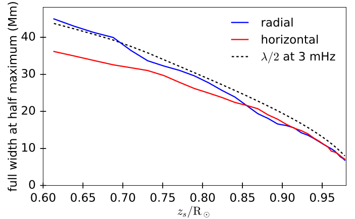
Fig. 5. Radial and horizontal widths of the frequency-averaged sound-speed kernel |\langle K^c \rangle| as functions of scattering position. These are close to half the local wavelength at 3 mHz (dotted line).
