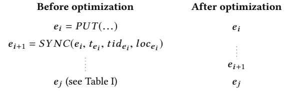
Figure 2: Code transformation for maximal overlap with respect to local dependencies.
