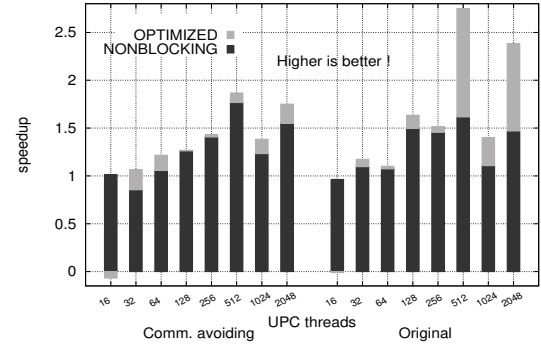
Figure 8: Speedup in communication when using nonblocking communication and our optimized version delaying synchronizations into nonblocking barriers of miniGMG, IMM version, (weak scaling). Results obtained on Edison.
