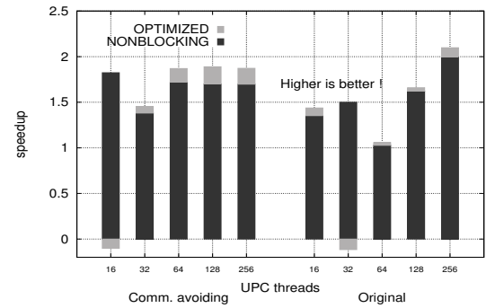
Figure 10: Speedup in communication when using nonblocking communication and our optimized version of miniGMG, AGG version PC (weak scaling). Results obtained on Shepard.
