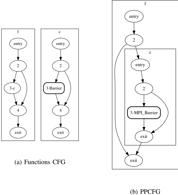
Fig. 2: MPI Code 4 functions CFG (left) and the corresponding PPCFG (right)
