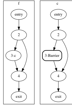
(a) Functions CFG
