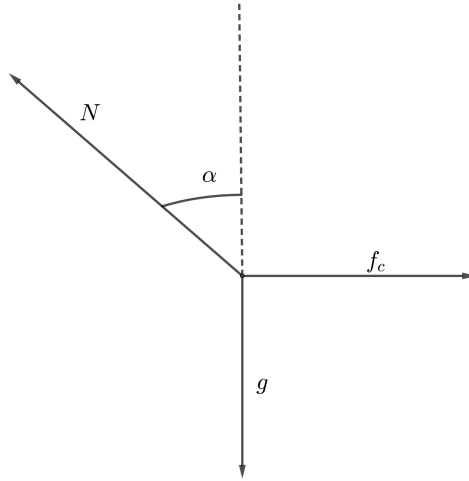
Figure 1. Illustration of the forces on the runner
