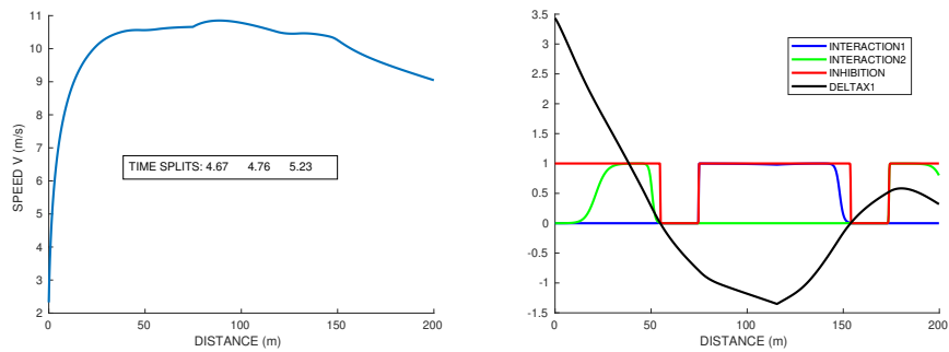
Figure 9. Race A_1 vs himself at lanes 5-4, with interaction \gamma = 0.04 and inhibition \eta = 20m . Left graph: speed profile and time splits of the runner at lane 5. Right graph: distance gap and interaction term for both runners. The sign changes of the distance gap correspond to the 2 overtakings.
