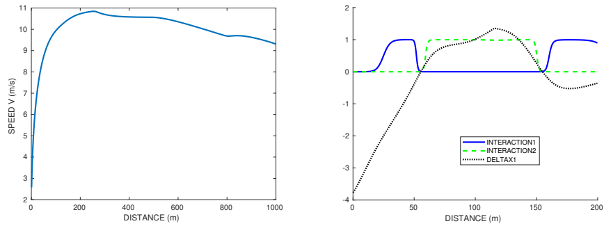
Figure 7. Race A_1 vs himself at lanes 1-2, with interaction \gamma = 0.04 and a frame \eta = 0 that is no inhibition. Left graph: speed profile and time splits of the runner at lane 1. Right graph: distance gap and interaction term for both runners. The sign change of the distance gap corresponds to the overtaking. Lane 2 wins by 0.04s.
