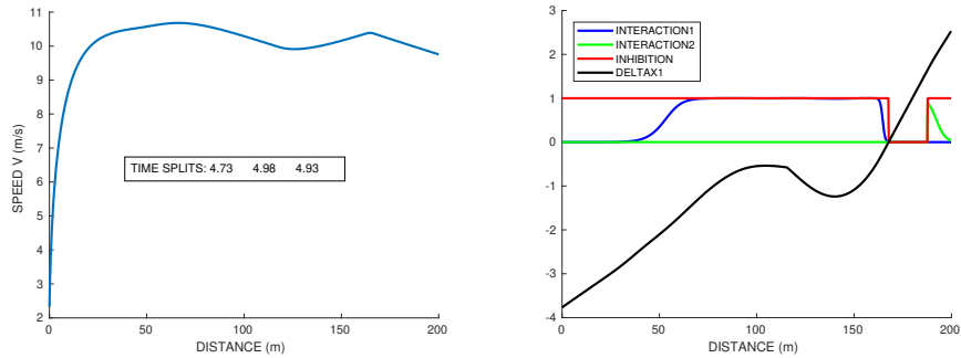
Figure 8. Race A_1 vs himself at lanes 1-2, with interaction \gamma = 0.04 and a frame \eta = 20m for the inhibition. Left graph: speed profile and time splits of the runner at lane 1. Right graph: distance gap and interaction term for both runners. The sign change of the distance gap corresponds to the overtaking. Lane 1 wins by 0.27s.
