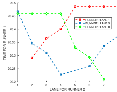
Figure 10. Times for athlete A_1 at lanes 1,5,8, running against himself.
