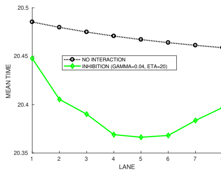
Figure 11. Mean times per lane for runner A_1 when in lane i vs himself in all other lanes. Without interaction ( \gamma = 0 ), and with interaction \gamma = 0.04 , \eta = 20 . Lane performance (sorted by mean time): \bar{T}_5 < \bar{T}_6 < \bar{T}_4 < \bar{T}_7 < \bar{T}_3 < \bar{T}_8 < \bar{T}_2 < \bar{T}_1 . Gap \bar{T}_1 - \bar{T}_8 = 0.050859 .
