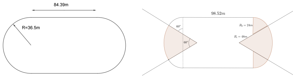
Figure 2. Shape for standard track (left) and double bend 2 track (right).
