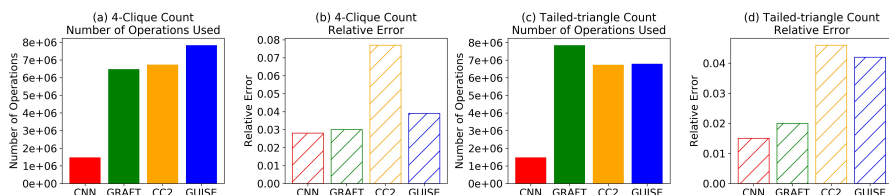
Fig. 1. Comparison of the number of arithmetic operations used for estimating 4-clique counts, tailed-triangle counts on 50-node ER graphs with edge existing probability 0.5. (a, c) The number of operations used by each framework. (b, d) The relative error each framework makes.
