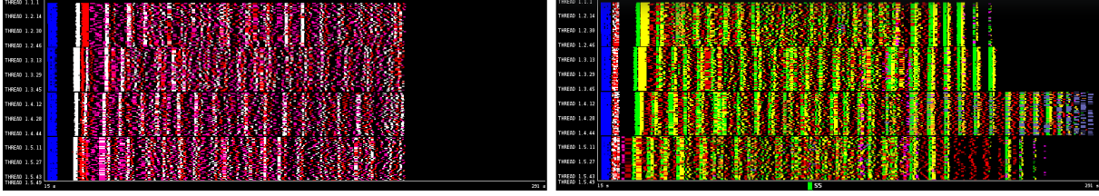
Figure 14. LU decomposition: Paraver trace. At left, userparallel and, at right, the autoparallel version
