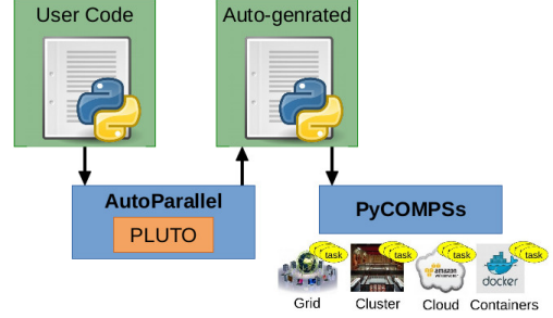
Figure 7. AutoParallel Module Overview
