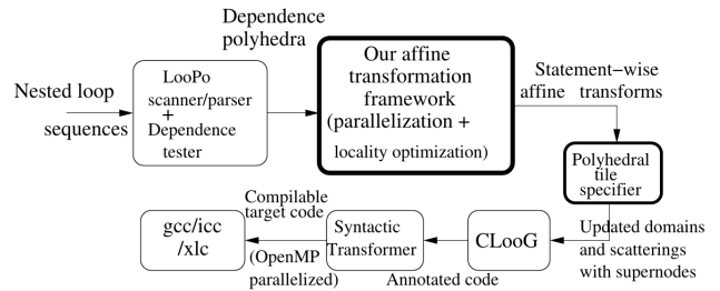
Figure 5. Pluto source-to-source transformation. Source: [28]
