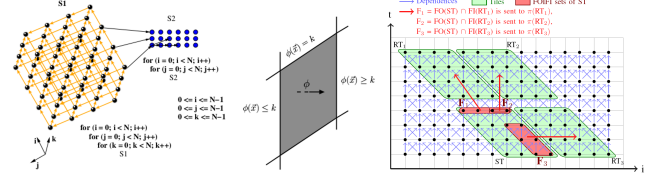
Figure 4. Pluto overview. Source: Pluto's official website [27]
