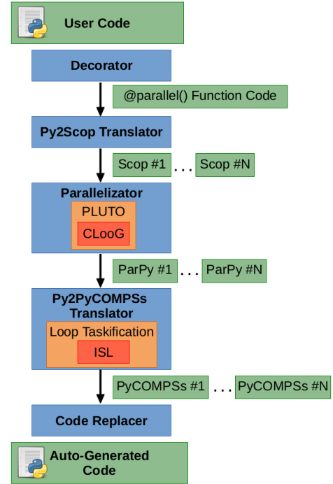
Figure 8. AutoParallel Module Internals
