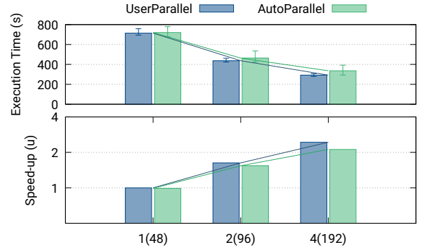
Figure 13. LU decomposition: Execution times and speed-up
