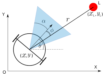
Fig. 2: A unicycle equipped with a fixed camera receives position measurements updates whenever a visual landmark (red dot) is close enough and enters the field of view.
