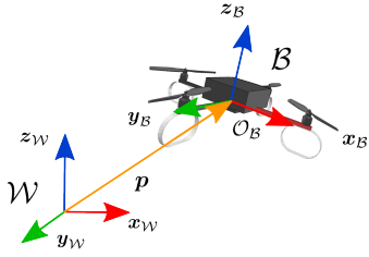
Fig. 3: Quadrotor model
