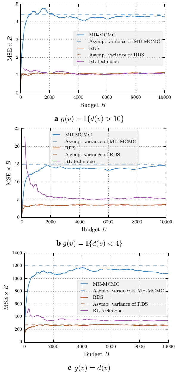
Fig. 4 Les Misérables network: asymptotic variance comparisons (theoretical and estimated)
