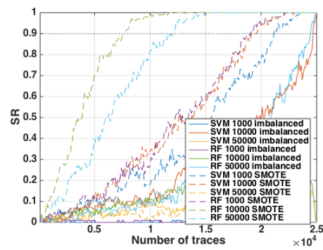
(f) Success rate (SR) on AES_HD.
