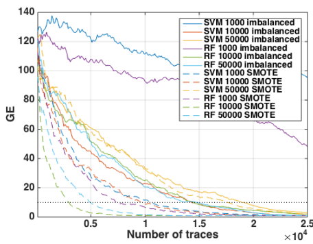
(e) Guessing entropy (GE) on AES_HD.
