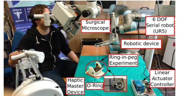
Fig. 6: Ring-in-peg experiment.
