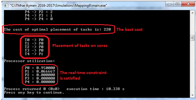
Fig. 2. Presentation of OptimalMappingTasks .
