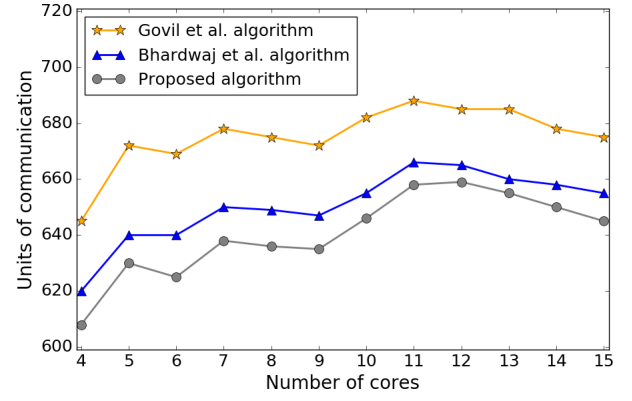
Fig. 8. Communication cost of our strategy when the cores are in an increasing order and the number of tasks is 50.
