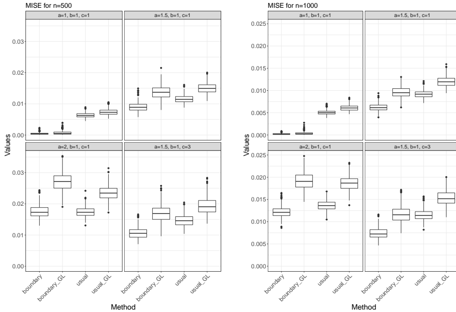
Figure 2: Boxplots of the integrated squared error (ISE) on the disk for the models described by Cases 1 to 4, and sample sizes equal to 500 and 1000 for the four estimators boundary , boundary_GL , usual and usual_GL .
