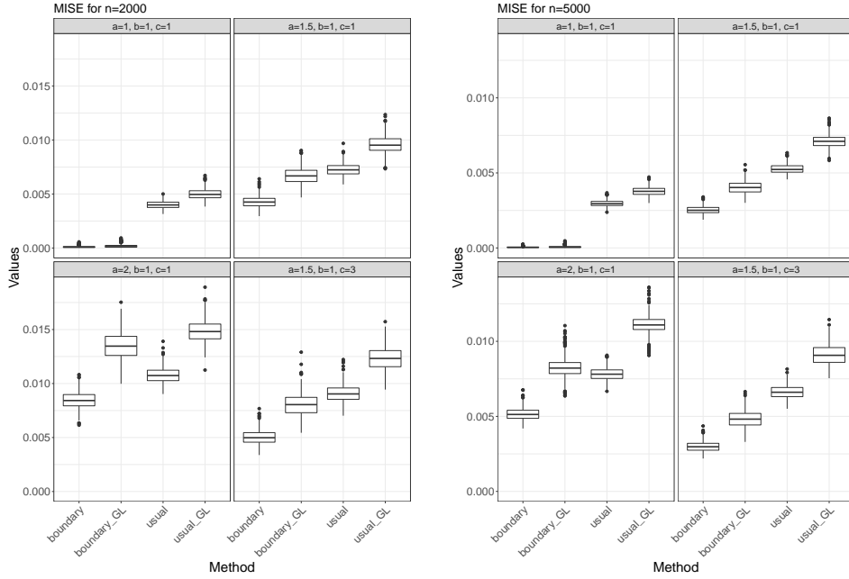
Figure 3: Boxplots of the integrated squared error (ISE) on the disk for the models described by Cases 1 to 4, and sample sizes equal to 2000 and 5000 for the four estimators boundary, boundary_GL, usual and usual_GL.
