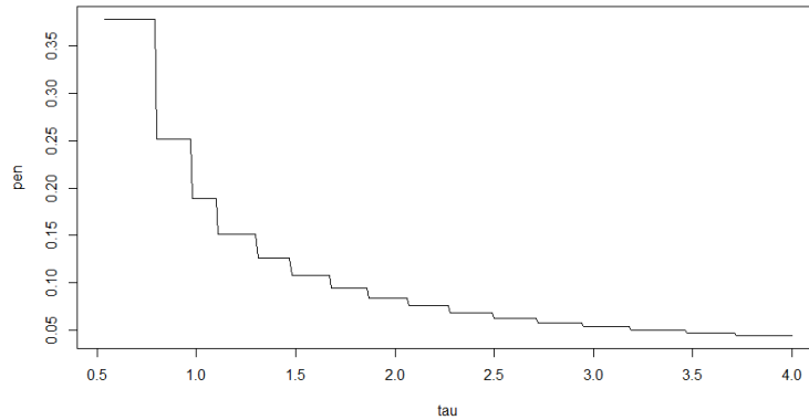
Figure 8: Value of the penalization \hat{M}(\hat{\ell}(\tau)) in terms of \tau .
