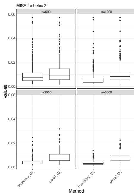
Figure 4: Boxplots of the integrated squared error (ISE) of the GL procedure based on the boundary estimator for \beta = 2 and different sample sizes, n = 500, 1000, 2000 and 5000.
