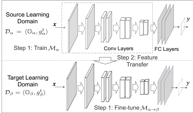
Figure 2: Transfer Learning with Convolutional Neural Networks.
