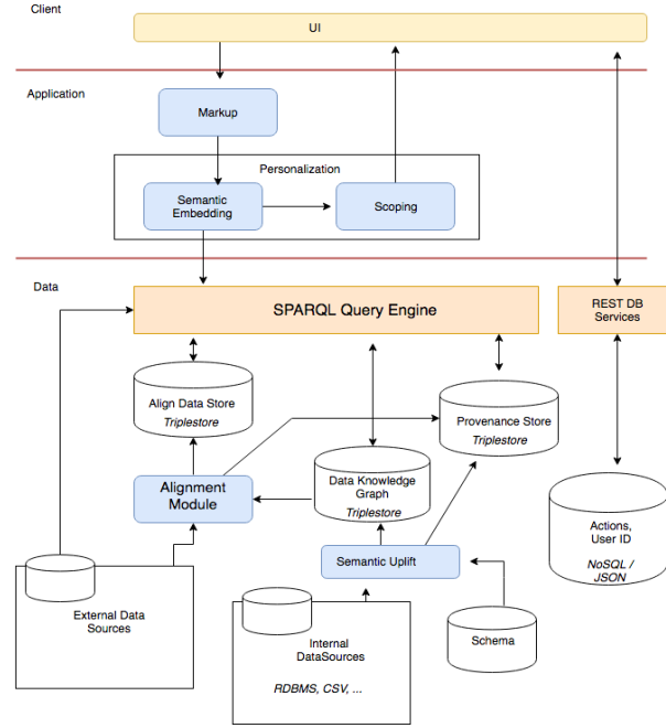
Fig. 1. The Architecture
