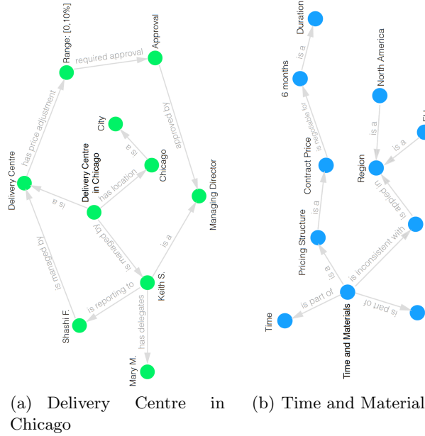
Fig. 4. Semantics-driven Representation of Context for Complex Terms of Action: “Adjust Time and Material for Delivery Centre in Chicago”.
