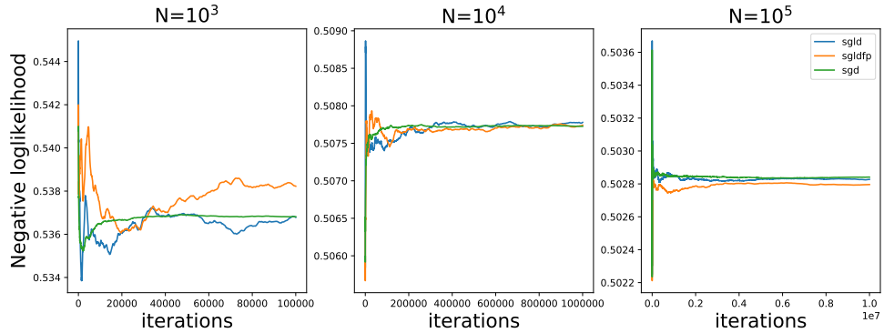
Figure 4: Negative loglikelihood on the test dataset for SGLD, SGLDFP and SGD function of the number of iterations for different values of N \in \{10^3, 10^4, 10^5\} .
