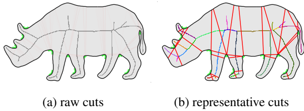
Fig. 10. (a) Symmetry : all cuts (in red, 95% transparent) whose endpoints are projections of the same interior medial axis point, with at least one endpoint on a concave corner. (b) Strong equivalence : representative cuts (in red) are selected such that for each corner there are at most two cuts (one double and one single) per interior medial axis branch. Corners and branches are shown in green and random color respectively.
