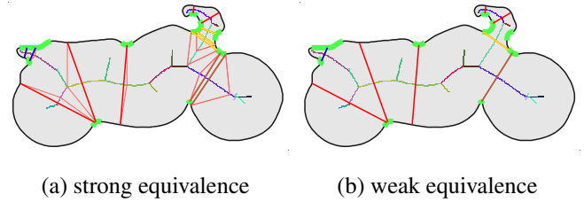
Fig. 11. Weak equivalence : representatives of (a) strong and (b) weak equivalence classes. In (a), cuts in blue, yellow and brown form three weakly equivalent classes, while the remaining representatives are in red. In the blue and brown class there are only two cuts (one double and single), while in the yellow class there are three cuts (two double and one single). In (b), we select the double cut as representative of the blue and brown class. For the yellow class, we select the double cut having the maximum number of votes. Corners and branches are shown in green and random color respectively. Pink lines connect cut points to their projections.
