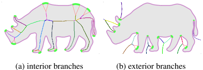
Fig. 7. (a) Interior branches from convex corners and interior boundary components. (b) Exterior branches from concave corners and exterior boundary components. Boundary components, corners and branches are shown in purple, green and random color respectively. Pink lines connect end-vertices to their projections.
