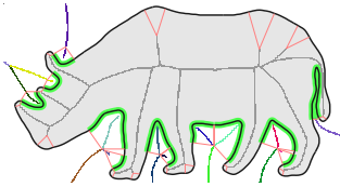
Fig. 8. Extended corners, in green. Pink lines connect the end-vertices of the interior medial axis to their projections and the last visited points in the backward traversal of the exterior medial axis to their projections. Branches of the exterior medial axis are shown in random color.
