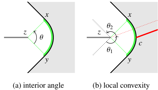
Fig. 6. (a) Interior angle \pi + \theta of a concave corner (in green) determined by exterior medial vertex z and its projection points x, y , where \theta is the angle between the two line segments from z to x, y . (b) By translating the two boundary segments starting at x, y and the cut (in red) starting at c to the same origin (vertex z here), shown as dotted lines, we measure the interior angles \theta_1, \theta_2 of the two shape parts at this corner after cutting. Both are less than \pi , while \theta_1 + \theta_2 is not. Local convexity is achieved and there is no need for more cuts at this corner. See section 7.
