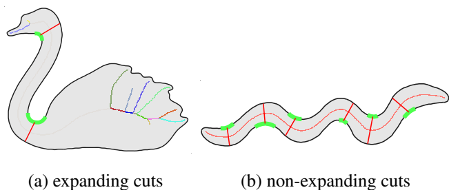
Fig. 15. (a) Expanding single cuts are not discarded. (b) Non-expanding single cuts are discarded. All cuts are shown in red. Corners and branches are shown in green and random color respectively.
