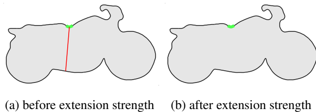
Fig. 16. Cuts lying on an extended corner (a) before and (b) after discarding according to extension strength. Cuts are shown in red and extended corners in green.
