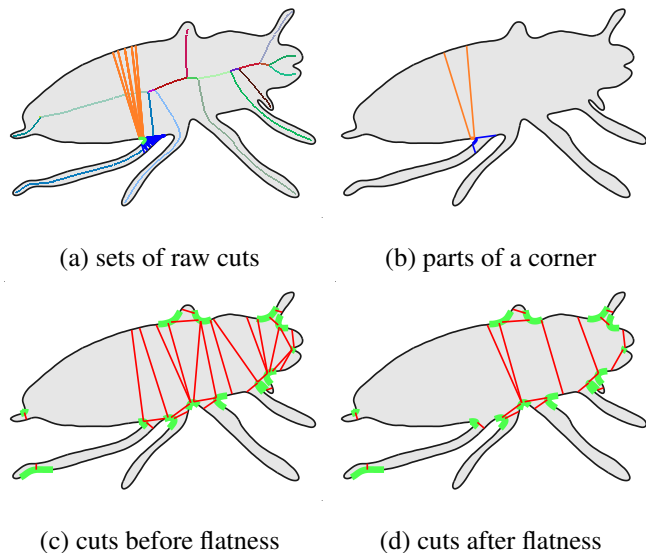
Fig. 14. (a) Two sets of raw cuts lying on a corner, shown in orange and blue. The corresponding cut points lie on two different branches. Branches are shown in random colors. (b) The two selected raw cuts from each set and the corresponding parts of the corner, shown again in orange and blue. Cuts (in red) (c) before and (d) after discarding according to flatness. Corners are shown in green.
