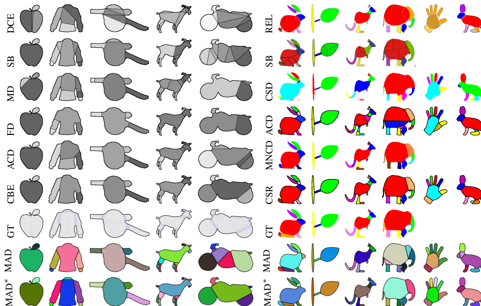
Fig. 19. Qualitative results on representative shapes of S&V De Winter and Wagemans (2006) (left) and Kimia Siddiqi and Kimia (1995) (right) datasets for a number of methods. Examples of competing methods on S&V are taken from Lewin et al. (2012a). Examples of competing methods on Kimia dataset are taken from the respective publications. Ground truth (GT) is depicted with cuts of all subjects overlaid in blue, 85% transparent, as in Fig. 9c.
