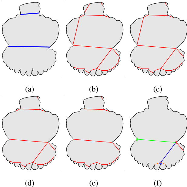
Fig. 17. Local convexity . (a) Majority cuts of shape #063 from S&V dataset. (b) Cuts (in red) before applying the local convexity rule. (c) Final selection of cuts without penalization and prioritization only according to short-cut rule, as in Papanelopoulos and Avrithis (2015). It is clear that more cuts are selected than what would be needed to achieve local convexity at each corner. (d) Final cuts with prioritization as defined in section 7.1. (e) Final cuts with priorities initialized as in section 7.1 and dynamically updated by penalization as discussed in section 7.2. Less cuts are selected comparing to (c). (f) The penalization process. All illustrated cuts have the same priority. The blue corner precedes the red one and as a result cuts lying on it are examined first. When we select the two orange cuts for the blue corner, local convexity is already achieved. If we did not penalize the blue cut, we would eventually select the red and blue cut to achieve local convexity at the red corner, because these cuts are shorter. With penalization, we rather select the green and red cut for the red corner. This works because corners far away from the shape center are examined first.
