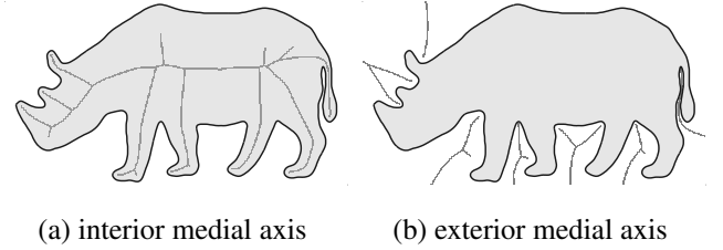
Fig. 2. Medial axes of shape #186 from S&V dataset De Winter and Wagemans (2006) which we use in experiments of section 8. (a) Interior medial axis. (b) Exterior medial axis.
