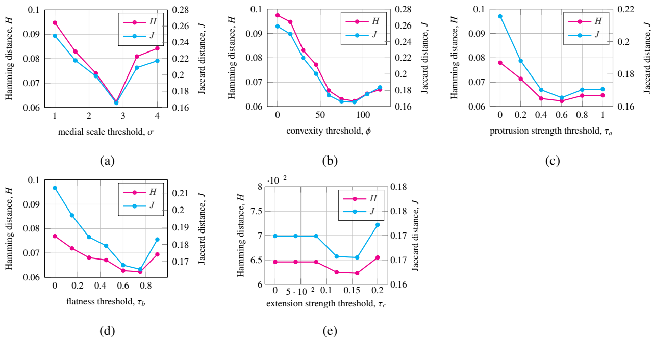
Fig. 18. Parameter tuning. Hamming ( H ) and Jaccard ( J ) distance vs. thresholds of (a) medial scale \sigma , (b) convexity \phi , (c) protrusion strength \tau_a , (d) flatness \tau_b , (e) extension strength \tau_c . Majority evaluation on S&V dataset. Lower is better for both evaluation measures. In each plot we fix the remaining parameters to their optimal value.
