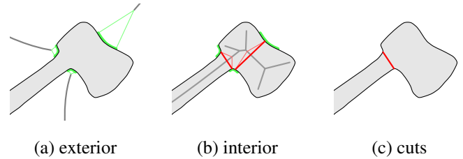
Fig. 1. Main elements of our method. (a) Minima rule : exterior medial axis and concave corners (in green) as boundary arcs that are each determined by one medial axis end vertex. (b) Symmetry : interior medial axis and candidate cuts (in red) whose endpoints are contained in corners and are projection points of the same medial axis point; only one such cut is selected per corner and medial axis branch. (c) Convexity rule : cuts are prioritized and selected for each corner such that each shape part is locally convex at the corner, roughly forming an interior angle less than \pi (up to tolerance).
