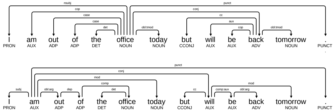
Figure 1: UD and SUD analysis of the same sentence (UD_English-EWT@2.2 email-enronsents38_01-0114 )
