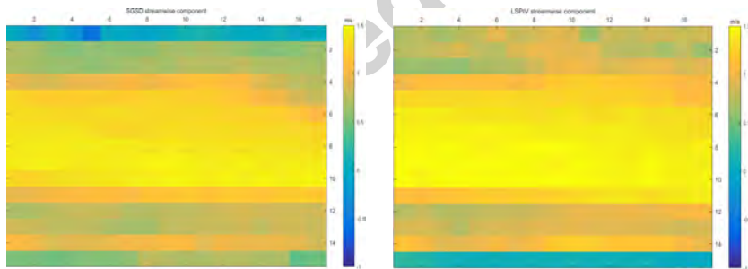
Figure 5.13: Real world velocity estimations on grid points, SGSD (left), LSPIV (right)
