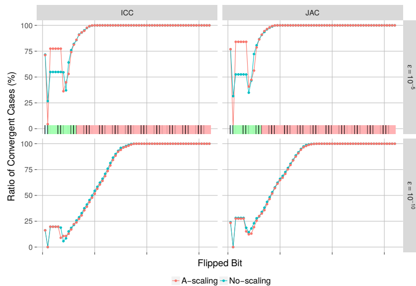
Figure 18: Impact of the index of the persistently flipped bit in the preconditioner application on PCG convergence success.
