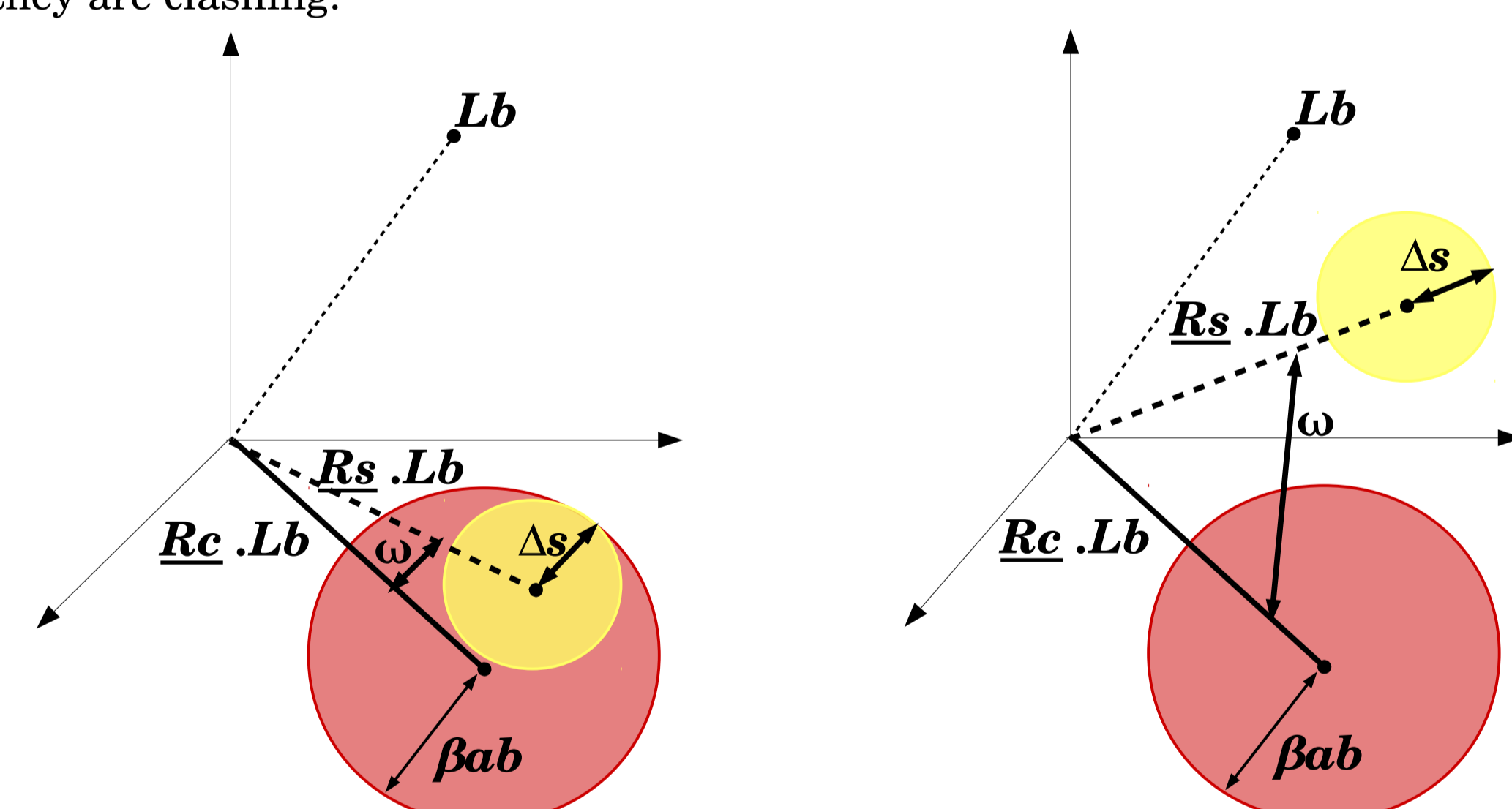
Case 1) \omega < \beta - \Delta_s \Rightarrow Every rotation within cube s cause a steric clash.
