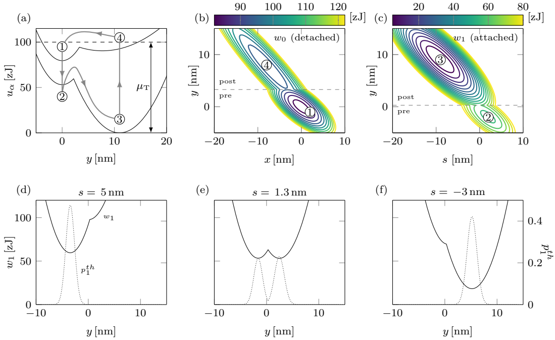
Fig. 2 (a) Representation of the bistable potential in the attached ( w_1 ) and detached ( w_0 ) states; the detached state is shown shifted by the amount of energy provided by ATP hydrolysis \mu_T and the gray line represents a typical Lymn-Taylor cycle with four stages (Lymn and Taylor 1971): (1) detached pre-, (2) attached pre- (3) attached post- (4) detached post-power-stroke. (b) and (c) Contours of the overall energy w_\alpha in the detached (b) and attached (c) states; the horizontal dashed lines show the position of the energy barrier between the pre- and the post-power stroke states. (d)–(f) overall energy w_1 (solid line) and equilibrium distribution (dotted line) in the attached state for different values of s .
