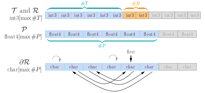
Fig. 10. The sets \mathcal{T} and \mathcal{R} are stored in a shared memory array of constant size \text{max} \#T , the variables \#T and \#R are the corresponding element counters. \mathcal{P} and \partial\mathcal{R} are also stored in shared memory arrays of constant size \text{max} \#P , and \#P is the number of stored plane equations.
