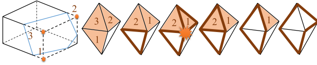
Fig. 11. Finding the boundary of \mathcal{R} : We initialize with the boundary of 1, and remove it from \mathcal{R} . We try to add the boundary of the new 1, but it would fail to produce a simple cycle. We try to add the boundary of 2 and it works, so we remove 2 from \mathcal{R} . Now we finish by adding the boundary of 1 and emptying \mathcal{R} .
