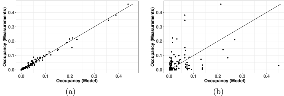
Figure 4: Model validation of occupancies for K = 1 : (a) multi-class and (b) two-class.
