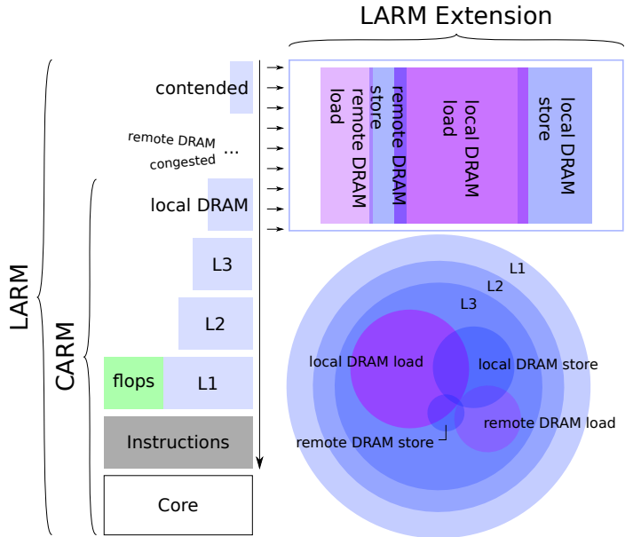
Fig. 14: LARM extension model compared with LARM and CARM models.
