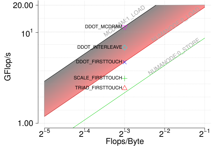
Fig. 13: Several STREAM benchmarks with different load/-store patterns and different memory allocations. Between MCDRAM:1_LOAD and NUMANODE:0_LOAD roofs is represented as a color gradient the possible scalar values for the hybrid roof depending on the physical memory access pattern between each hereby characterized memory.
