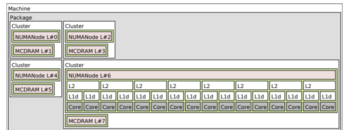
Fig. 7: hwloc model of KNL topology in SNC-4 flat mode. Only the fourth cluster is detailed, for simplifying representation. Other clusters have a similar topology.
