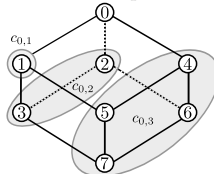
General c_{i,s} table for 8 nodes
