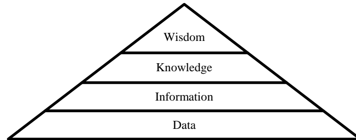
Fig. 1. Knowledge Hierarchy [18]
