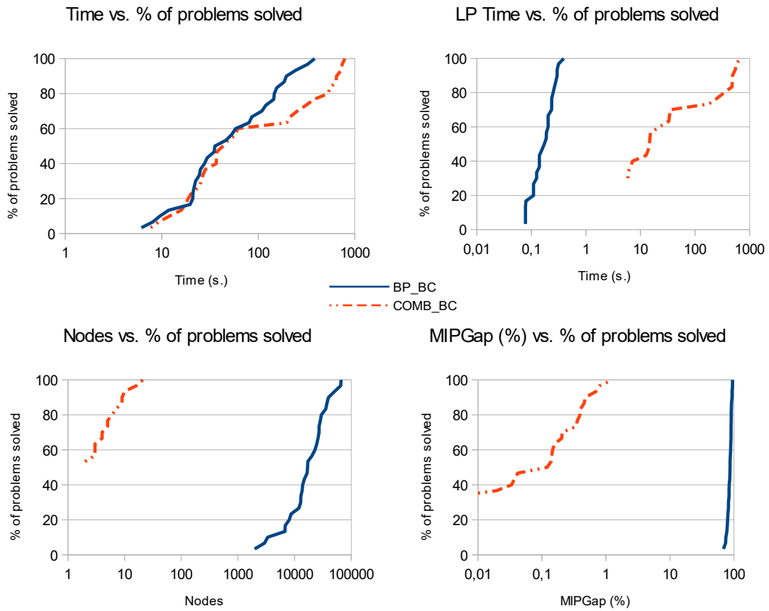
Figure 5 Performance profile graphs for instances with 10 security resources in graphs of up to 80 nodes
