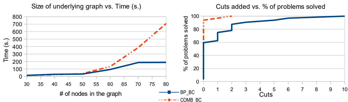
Figure 4 Instances with 10 security resources in graphs of up to 80 nodes
