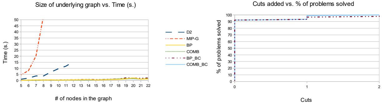
Figure 2 Instances with 2 security resources in graphs of up to 22 nodes
