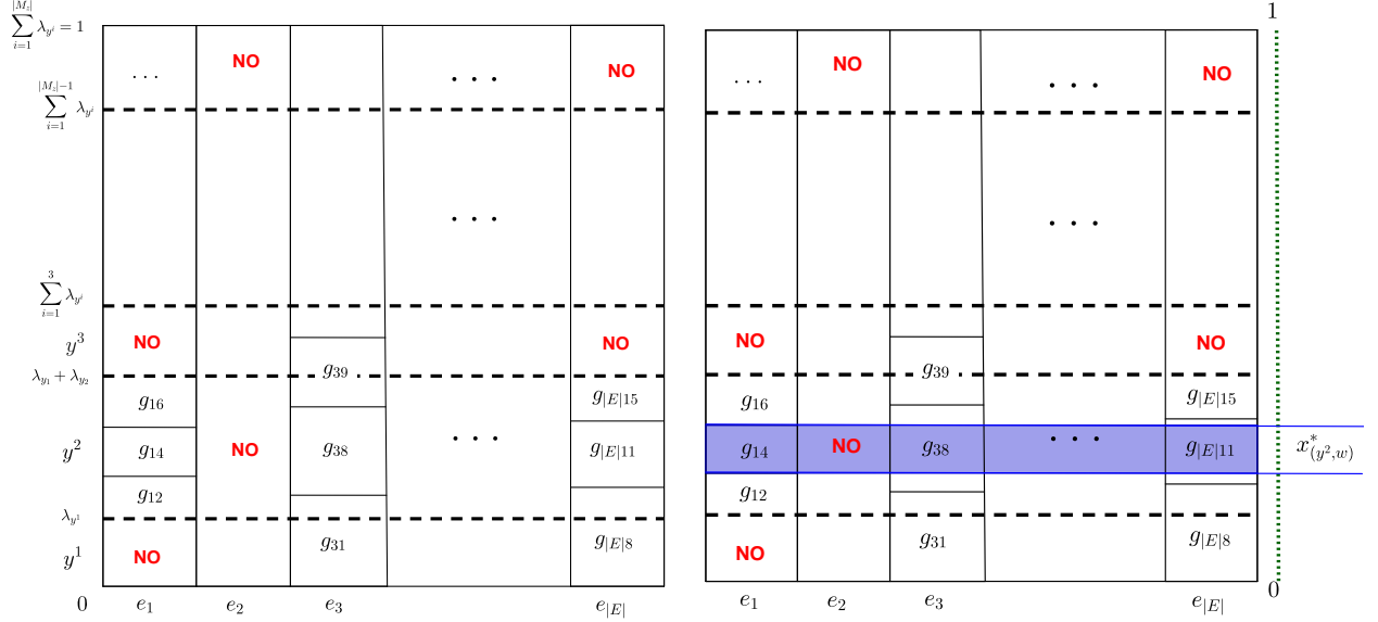
Figure 1 Construction to identify mixed strategy \mathbf{x} given feasible vectors \mathbf{z}, \mathbf{c}, \mathbf{g} . Here matching y^2 includes edges e_1, e_3, \dots, e_{|E|} . A constant width horizontal line (shaded) can be identified using portions of g_{14}, g_{38}, \dots, g_{|E|11} . This shaded horizontal line corresponds to using precinct pairings according to matching y^2 and protecting targets w = \{4, 8, \dots, 11\} , whose width we label as x_{(y^2, w)} .
