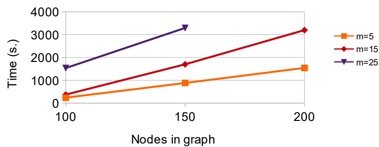
Figure 6 Solution times for (BP_BC) in instances with n = 100, 150, 200 and m = 5, 15, 25
