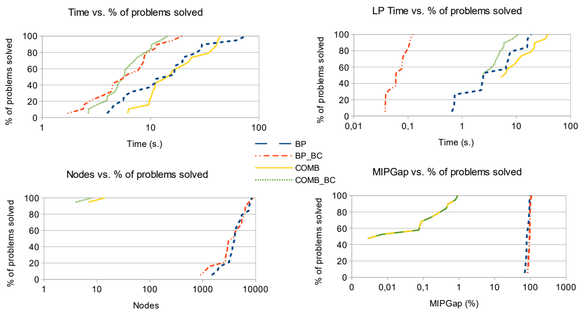
Figure 3 Performance profile graphs for instances with 4 security resources in graphs of up to 40 nodes
