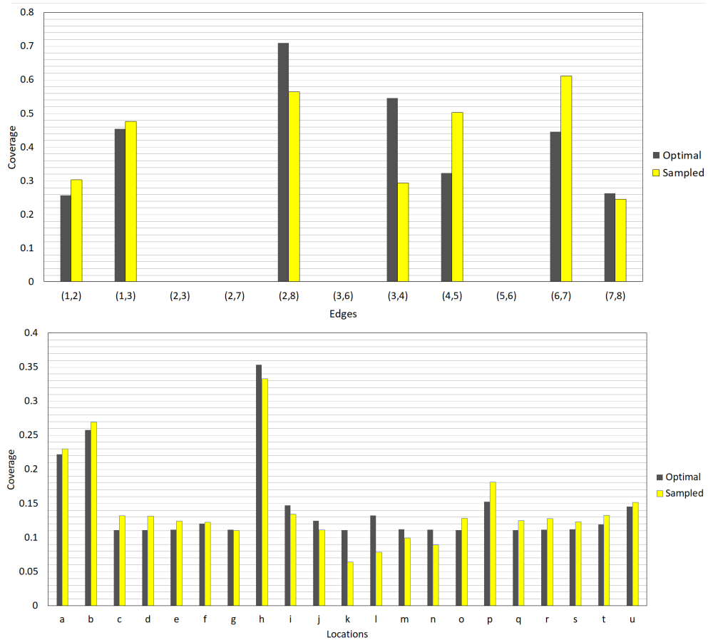
Figure 9 Coverage comparison in edges and targets in the realistic instance.
