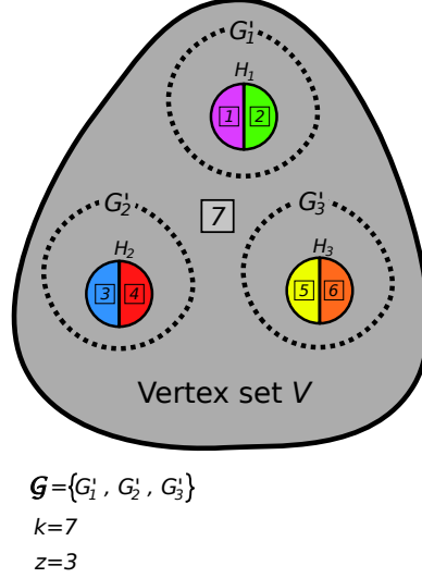
Figure 1: Illustration of the randomized labeling that achieves the lower bound in Theorem 7. The grey area includes all the nodes of V . In this example, we set z = 3 and k = 7 . In this case we thus have \lfloor \frac{k-1}{2} \rfloor = 3 . \mathcal{G} is the collection of the 3 vertex-disjoint subgraphs G'_1, G'_2 and G'_3 . The node set size of each of these subgraphs is equal to \lfloor \frac{n^2}{2m} \rfloor . The subsets of isolated vertices in these 3 subgraphs are H_1, H_2 , and H_3 , which are depicted in this figure by the bicoloured circles. Each color represents a class. For each j , the expected size of H_j must be linear in the size of the node set of G'_j . For j = 1, 2, 3 , set H_j is labeled by selecting uniformly at random a class between the two classes (or colors) 2j - 1 and 2j . All the remaining nodes in the grey area of this picture are given the same class 7. Hence, for each pair of nodes u and v both belonging to H_j for some j , we must have (u, v) \notin S . On the contrary, for each pair u and v with u \in H_j , for some j , and v \notin H_j , we must have y_{u,v} = 0 . The information of the training set cannot be used to predict how the nodes in H_1, H_2 , and H_3 , are labeled. In fact, any algorithm will make \frac{1}{2} mistakes in expectation over the randomized labeling on each node contained in these subsets.
