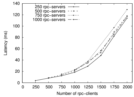
Fig. 3. Average Latency
