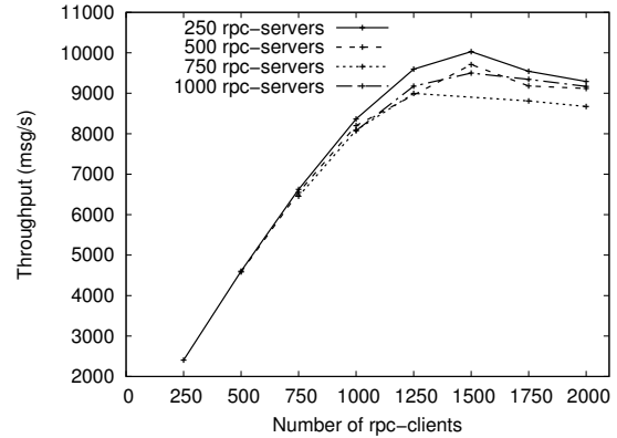
Fig. 4. Average Throughput
