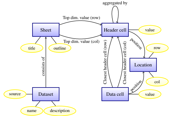
Figure 2: Conceptual data model.
