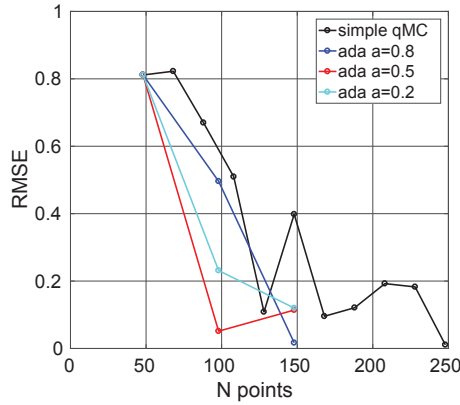
Figure 12: TEST 2: Convergence of the RMSE. The result of a simple increase of the qMC Halton set is compared with adaptation at different values of \alpha coefficient
