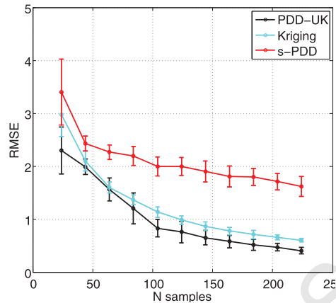
Figure 3: TEST 1: Mean RMSE convergence comparison between Ordinary Kriging, sparse PDD and coupled PDD-UK metamodels, m = 5
