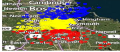
Fig. 2. Regionalization.
