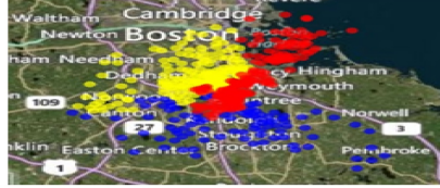
Fig. 12. K-means_{d_{Dyn2}}(\alpha = \beta = 0.5) .
