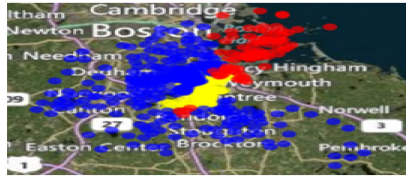
Fig. 3. Classical K-means.
