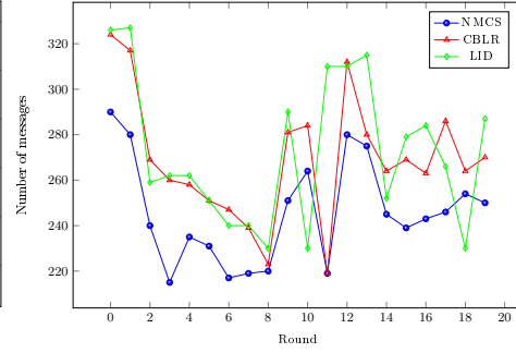
Fig. 6: Communication overhead comparison.
