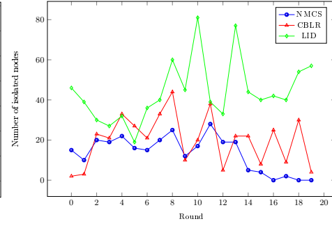
Fig. 4: Number of isolated nodes per round.
