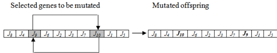
Fig. 3. Example of the mutation operator.
