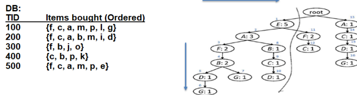
Fig. 1 Construction of FP-tree top-down and left-to-right
