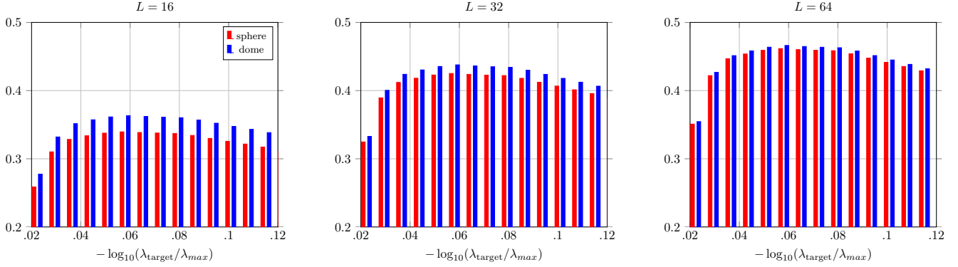
Figure 4. Computational savings (see (53)) induced by joint screening for different number of regions L and values of the regularization parameter.
