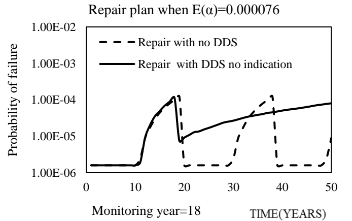
Figure 9. Repair plan during service life if implementing DDS at year 18 when expected mean deterioration rate is E(\alpha)=0.000073 .
