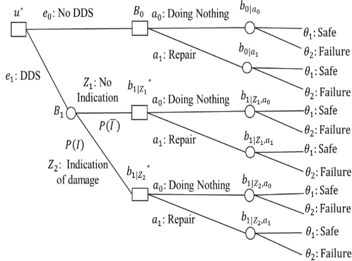
Figure 7. Illustration of decision tree combining a prior decision analysis and a pre-posterior decision analysis.
