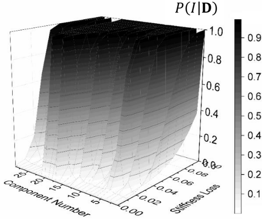
Figure 4. Probability of damage indication for 29 components in dependency of stiffness loss.
