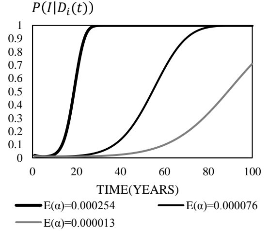
Figure 5. Probability of damage indication for one component during service life.
