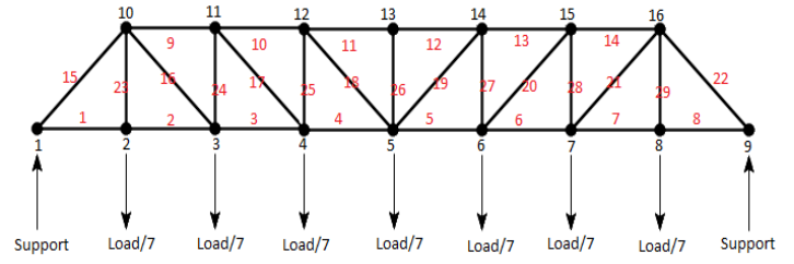
Figure 1. Pratt truss.
