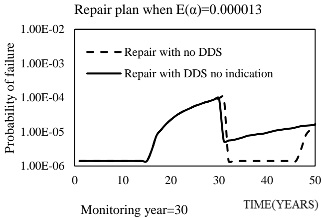
Figure 10. Repair plan during service life if implementing DDS at year 30 when expected mean deterioration rate is E(\alpha)=0.000013 .
