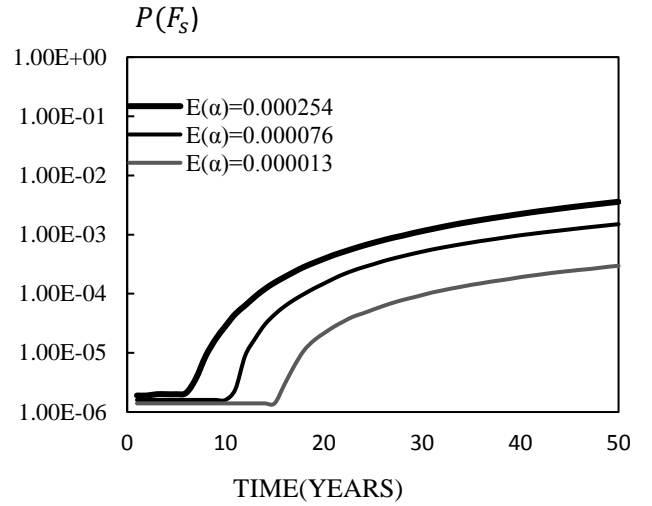
Figure 3. Prior probability of system failure in service life.
