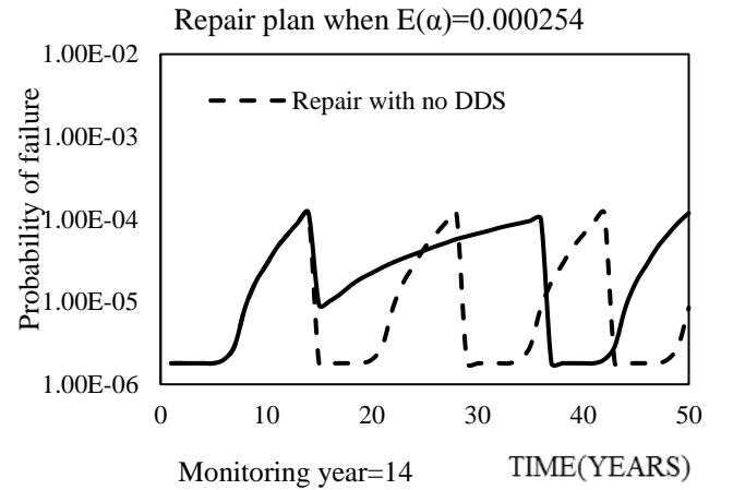
Figure 8. Repair plan during service life if implementing DDS at year 14 when expected mean deterioration rate is E(\alpha)=0.000254 .
