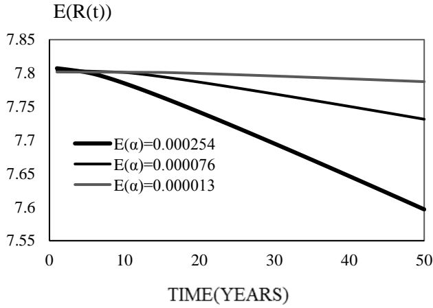
Figure 2. Expected resistance degradation in service life.
