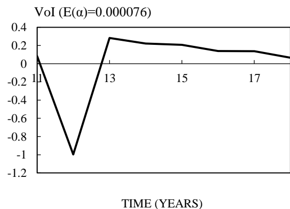
Figure 12. Value of DDS information independency of the DDS implement year when expected deterioration rate is E(\alpha)=0.000076 .
