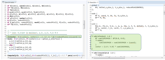
Figure 13. Example of Nabla Code Generation
