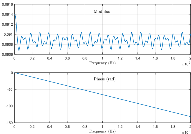
Fig. 5. S_{11}(\omega) after de-embedding.
