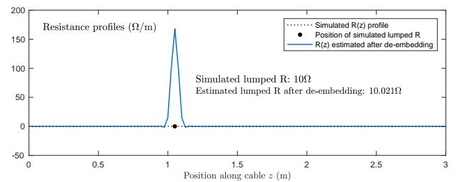
Fig. 7. Simulated cable resistance profile R(z) (uniform except a lumped R=10\Omega at z = 1.05\text{m} ), and estimated R(z) after de-embedding.
