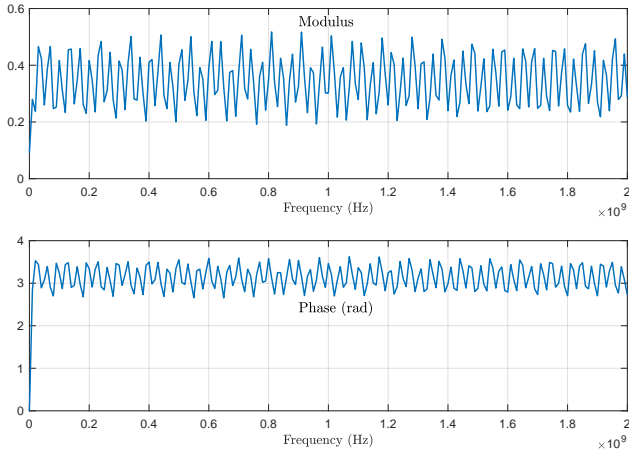
Fig. 4. S_{11}(\omega) with unmatched connectors (simulated with the P -matrix (14)) mounted on the simulated cable.
