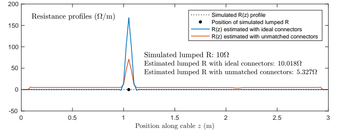
Fig. 6. Simulated cable resistance profile R(z) (uniform except a lumped R=10\Omega at z = 1.05\text{m} ), and estimated R(z) with data simulated with ideal connectors or with unmatched connectors.
