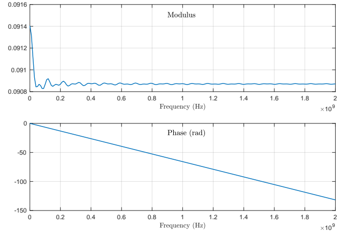
Fig. 3. S_{11}(\omega) with ideal connectors mounted on the simulated cable.
