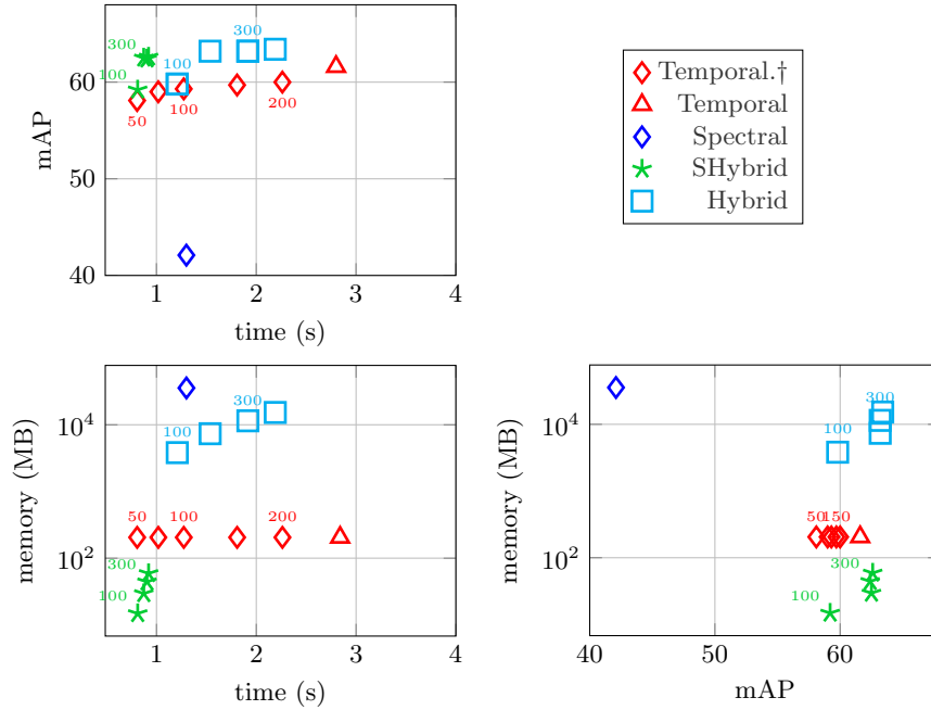
Fig. 5. Time (s) - memory (MB) - performance (mAP) for different methods. We show mAP vs. time, memory vs. time, and memory vs. mAP on \mathcal{R}Oxford + \mathcal{R}1M . Methods in the comparison: temporal for 20 iterations, truncated temporal for 20 iterations and shortlist of size 50k, 75k, 100k, 200k and 300k, spectral (FSRw) with r = 5k , hybrid with r \in \{100, 200, 300, 400\} and 5 iterations, sparse hybrid with 99% sparsity, r \in \{100, 200, 300, 400\} and 5 iterations. Text labels indicate the shortlist size (in thousands) for truncated temporal and rank for hybrid. Observe that the two plots on the left are aligned horizontally with respect to time, while the two at the bottom vertically with respect to memory.
