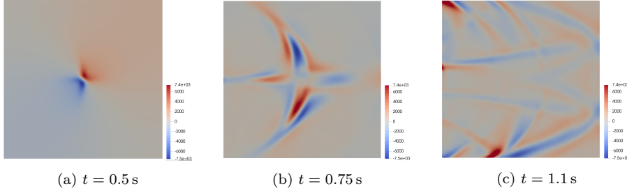
Fig. 12: Elastic wave propagation in a heterogeneous transverse isotropic medium (absolute value of the pressure field).
