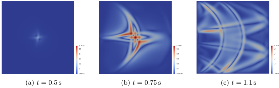
Fig. 11: Elastic wave propagation in a heterogeneous transverse isotropic medium (absolute value of the displacement field).
