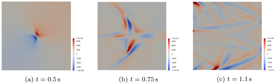
Fig. 12: Elastic wave propagation in a heterogeneous transverse isotropic medium (absolute value of the pressure field).
