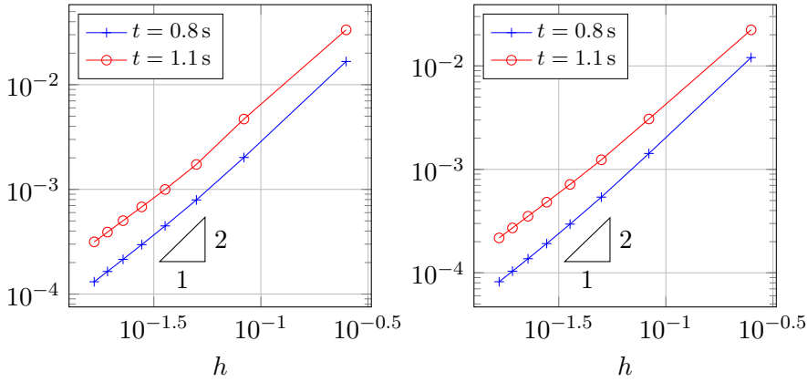
Fig. 10: Convergence of scheme (QIP) w.r.t. the space step h , for final time t = 0.8\text{ s} , t = 1.1\text{ s} for a heterogeneous transverse isotropic material. Left: L^2(H^1(\Omega)) -error on the displacement. Right: L^\infty(H^1(\Omega)) -error on the displacement.
