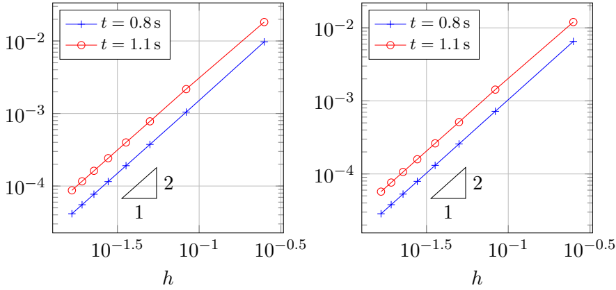
Fig. 9: Convergence of scheme (QIP) w.r.t. the space step h , for final time t = 0.8\text{ s} , t = 1.1\text{ s} for a heterogeneous transverse isotropic material. Left: Relative L^2(L^2(\Omega)) -error on the displacement. Right: Relative L^\infty(L^2(\Omega)) -error on the displacement.
