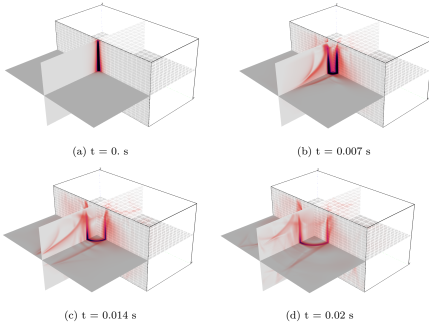
Fig. 13: Elastic wave propagation in a three-dimensional transverse isotropic medium (absolute value of the displacement field).
