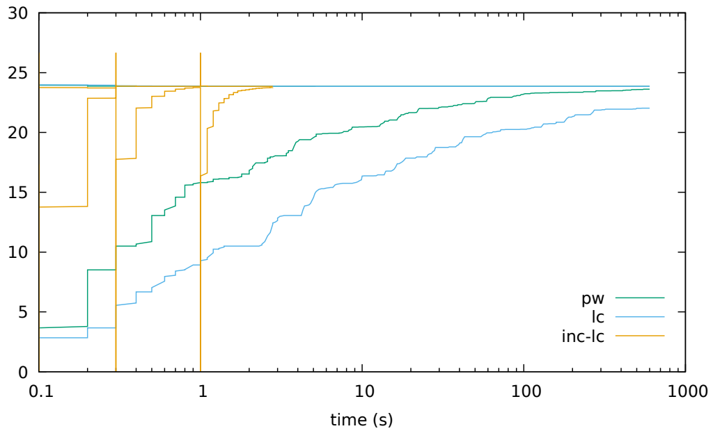
Figure 20: grid-info kx
